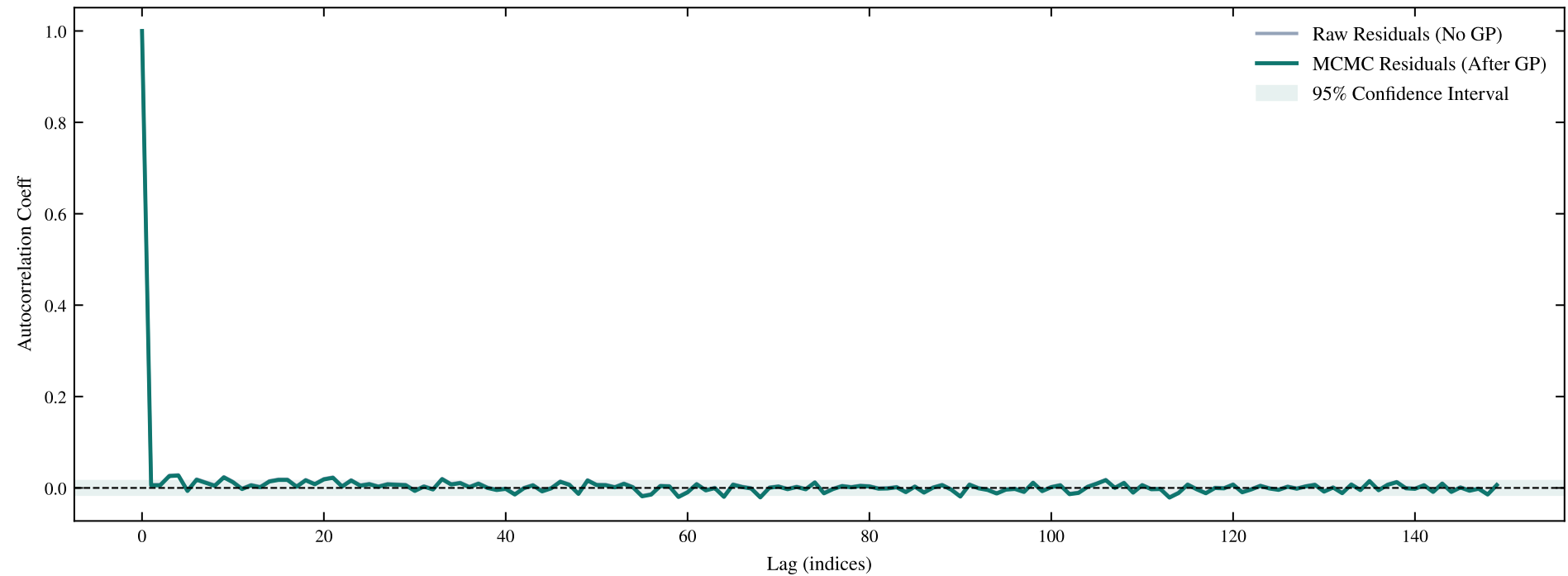
TIC 427508467 | Sectors: 34 | GP Residuals Autocorrelation Function (ACF)
