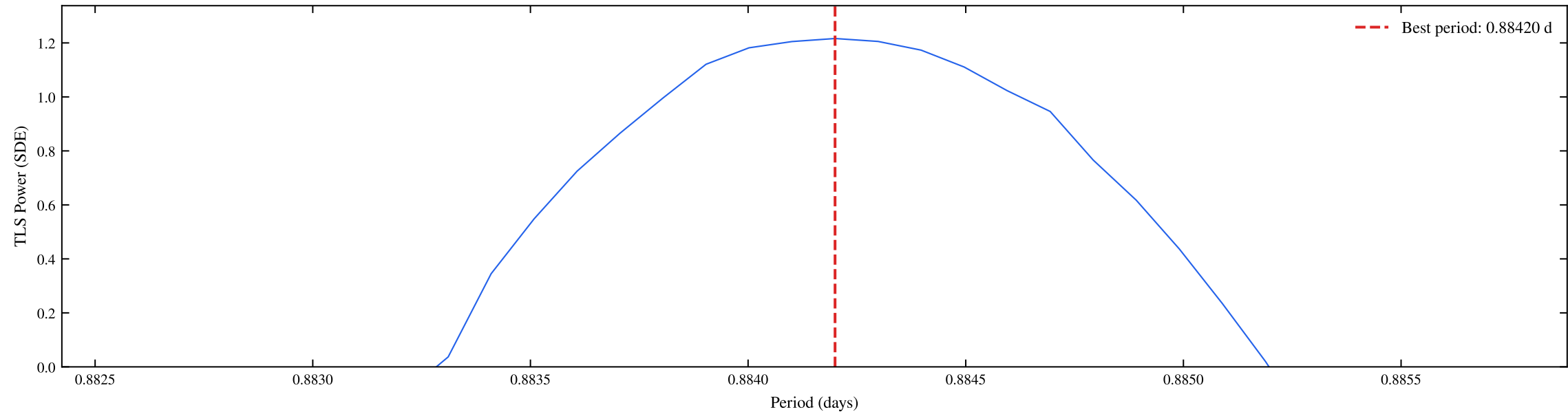
TIC 427508467 | Sectors: 34 | TLS Coarse Periodogram (SDE = 1.22)
