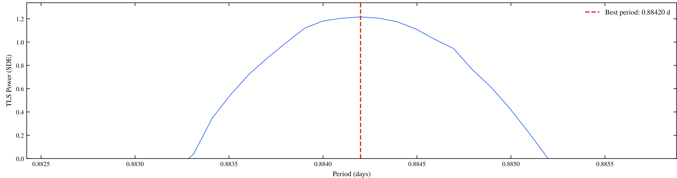
TIC 427508467 | Sectors: 34 | TLS Periodogram (SDE = 1.22)
