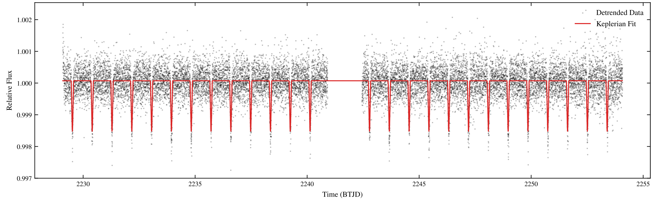
Detrended Light Curve & Best-Fit Transit Model
